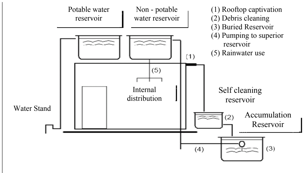
Figure 4. Rainwater use system in an urban lot [11].
