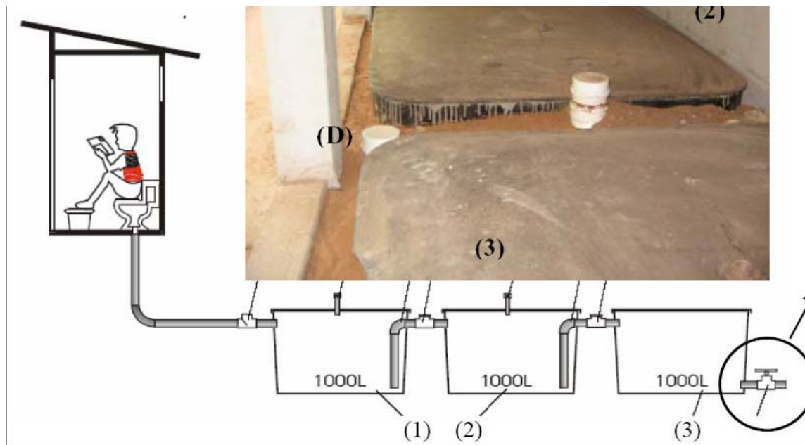
Figure 3. Scheme of the biodigesting patent concrete cesspit and pictures of the boxes (1), (2) e (3). [11]
