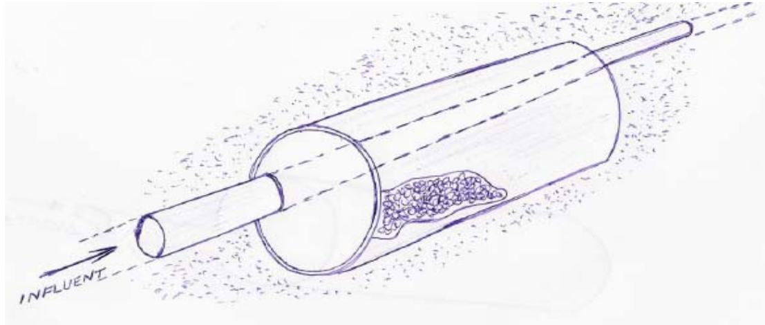
Figure 1 – Buried ecochamber destined to the dispersion of treated sanitary wastewater in the trees' roots. In the detail, the internal filling of the buried ecochamber can be seen with sequoia bark, which allows a closer contact of the liquid phase with the roots of the trees.
